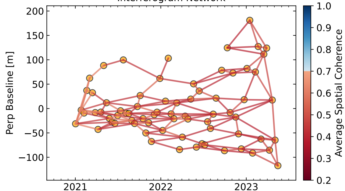
Interferogram Network
