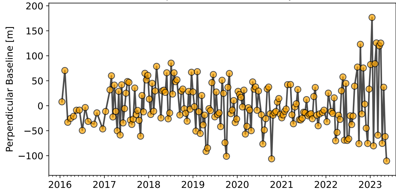
Perpendicular Baseline History
