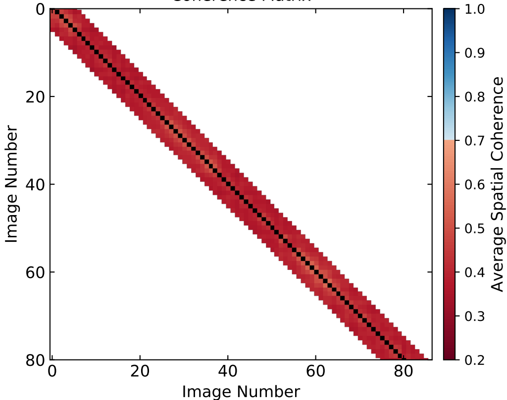
Coherence Matrix
