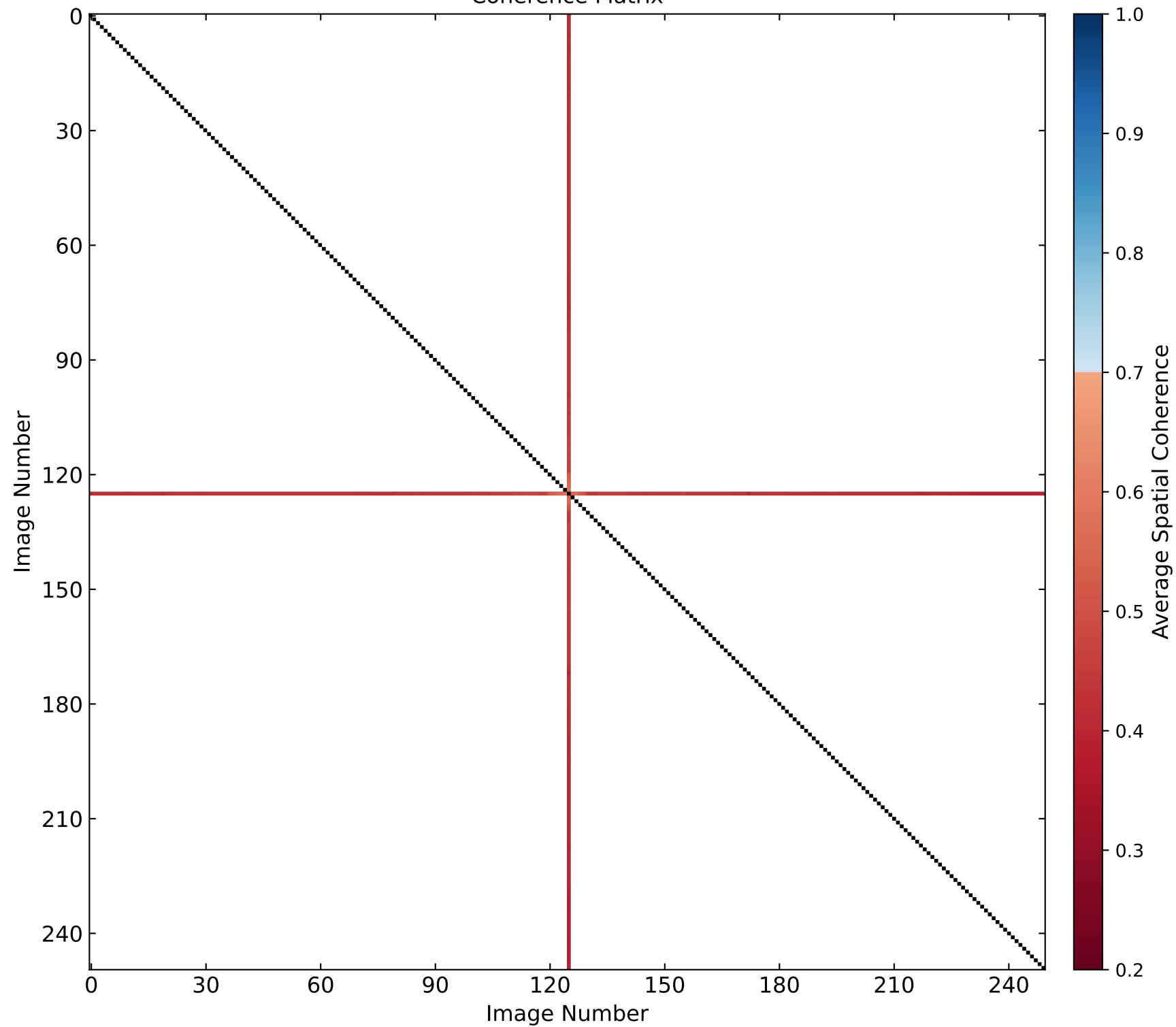
Coherence Matrix
