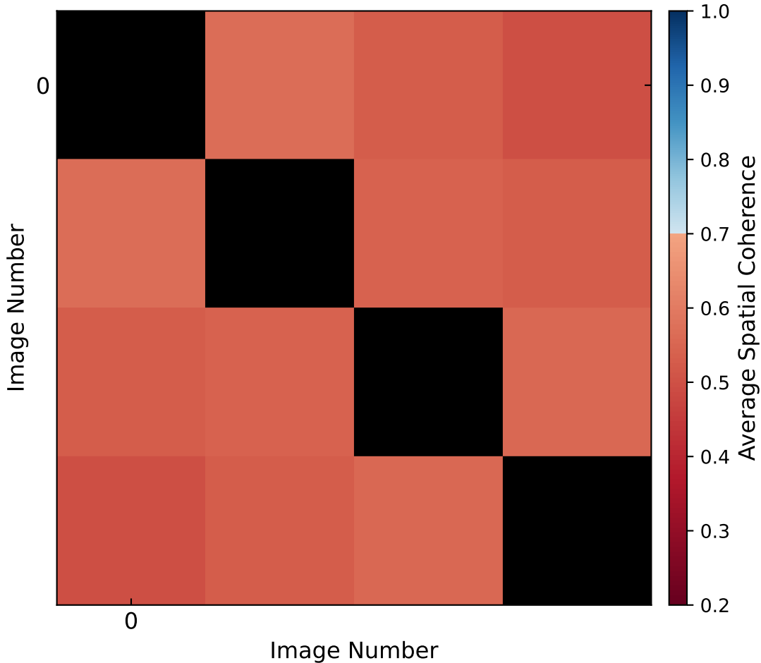
Coherence Matrix
