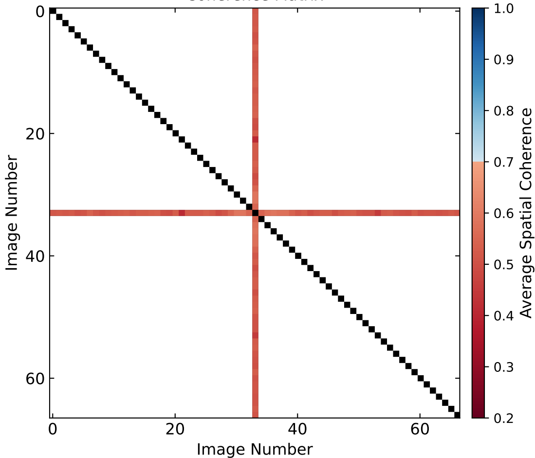
Coherence Matrix
