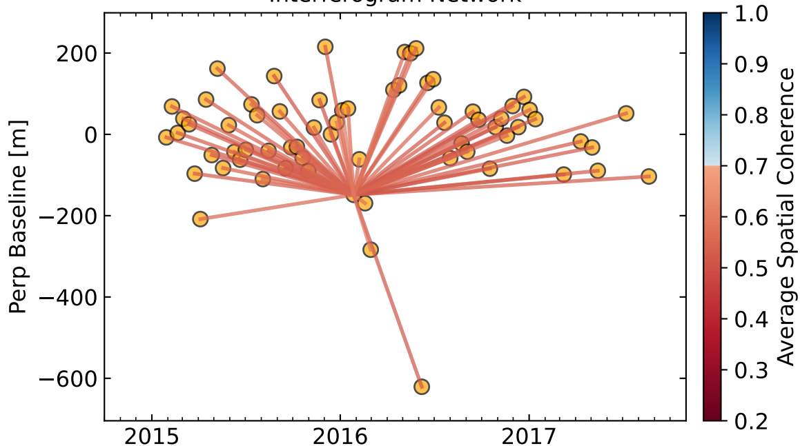
Interferogram Network
