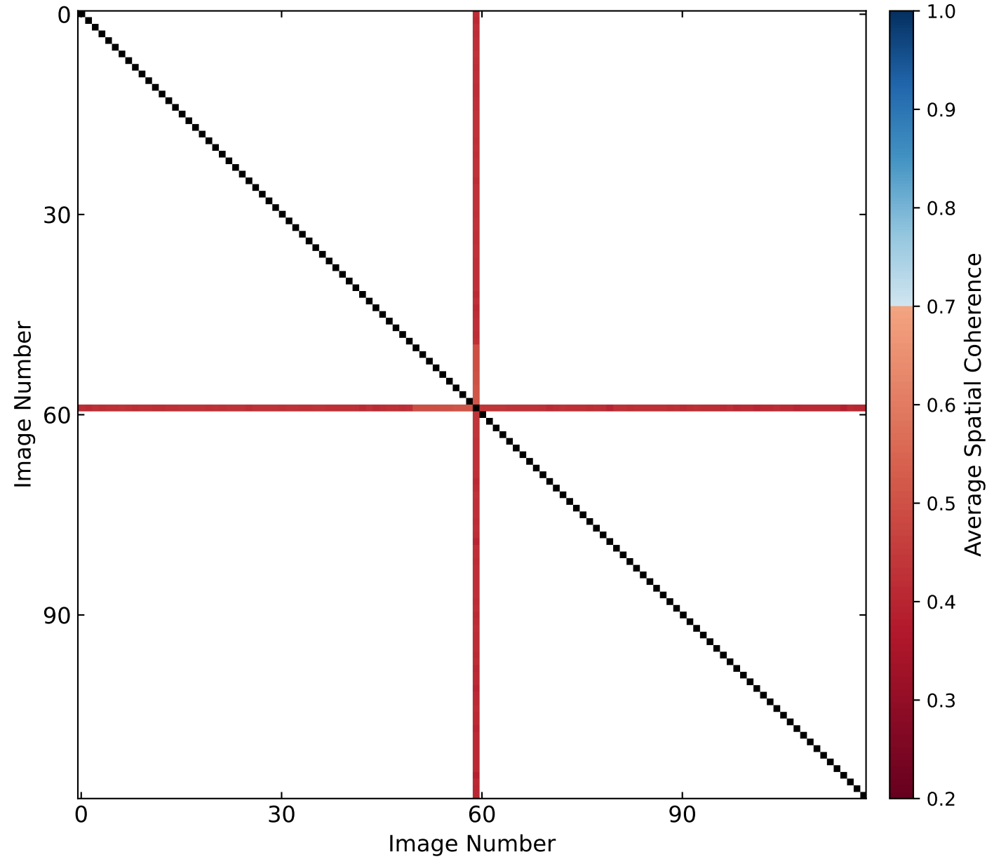
Coherence Matrix
