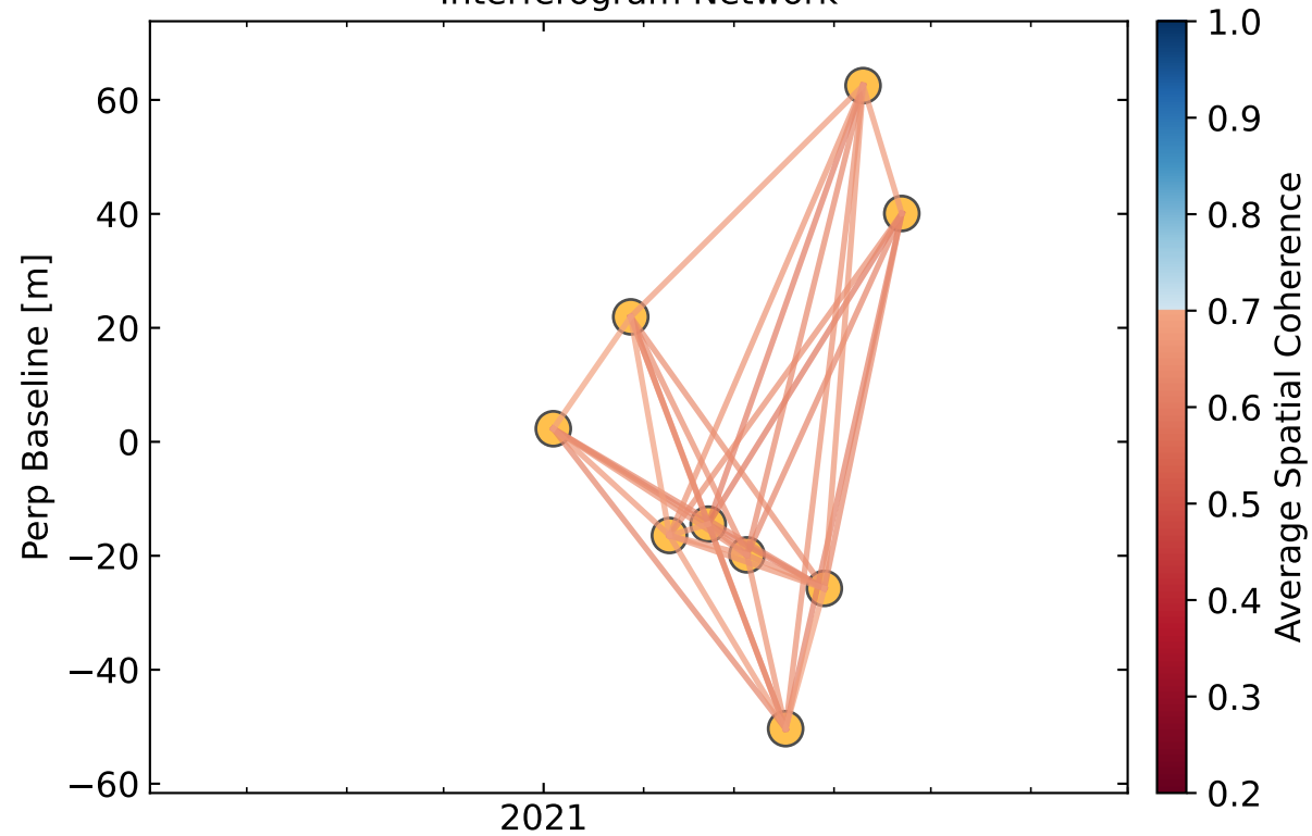
Interferogram Network
