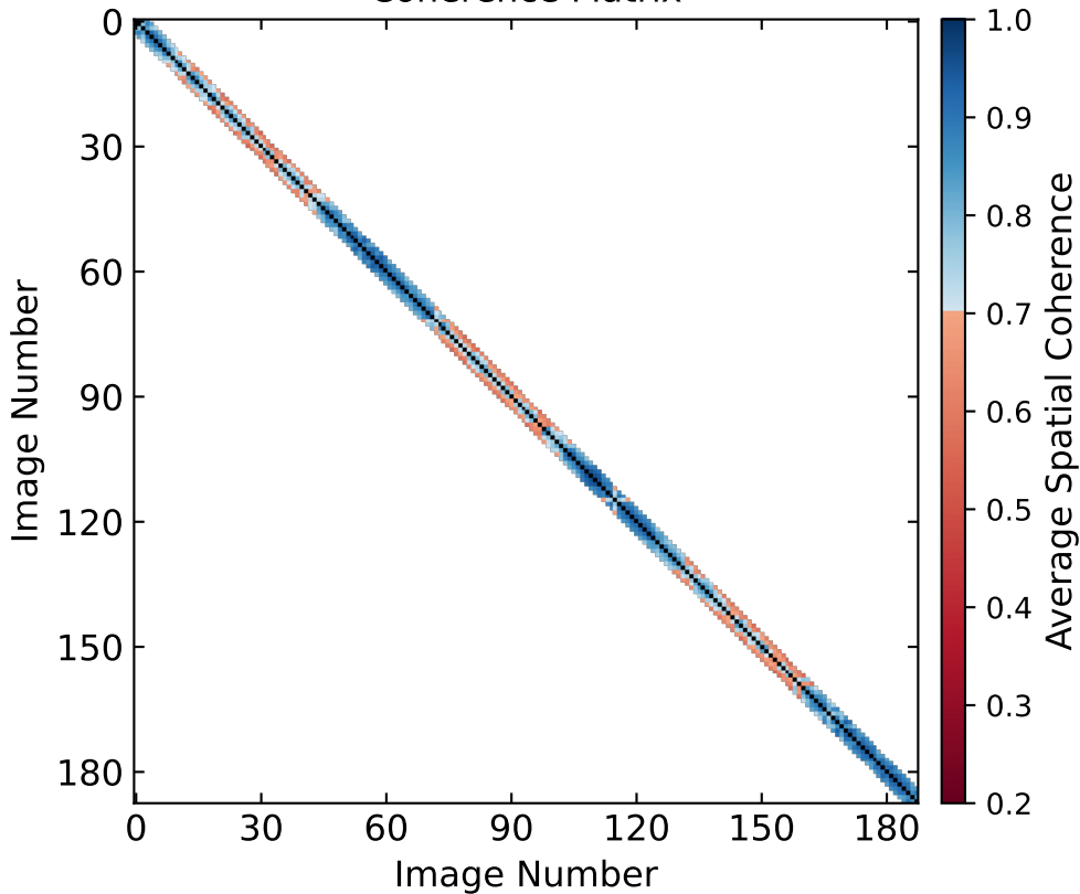
Coherence Matrix
