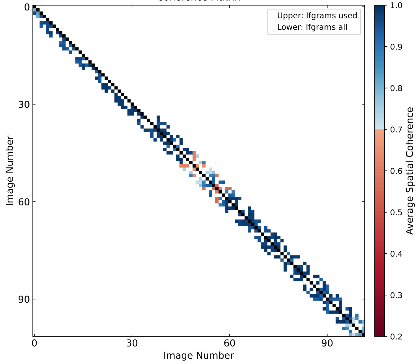
Coherence Matrix
