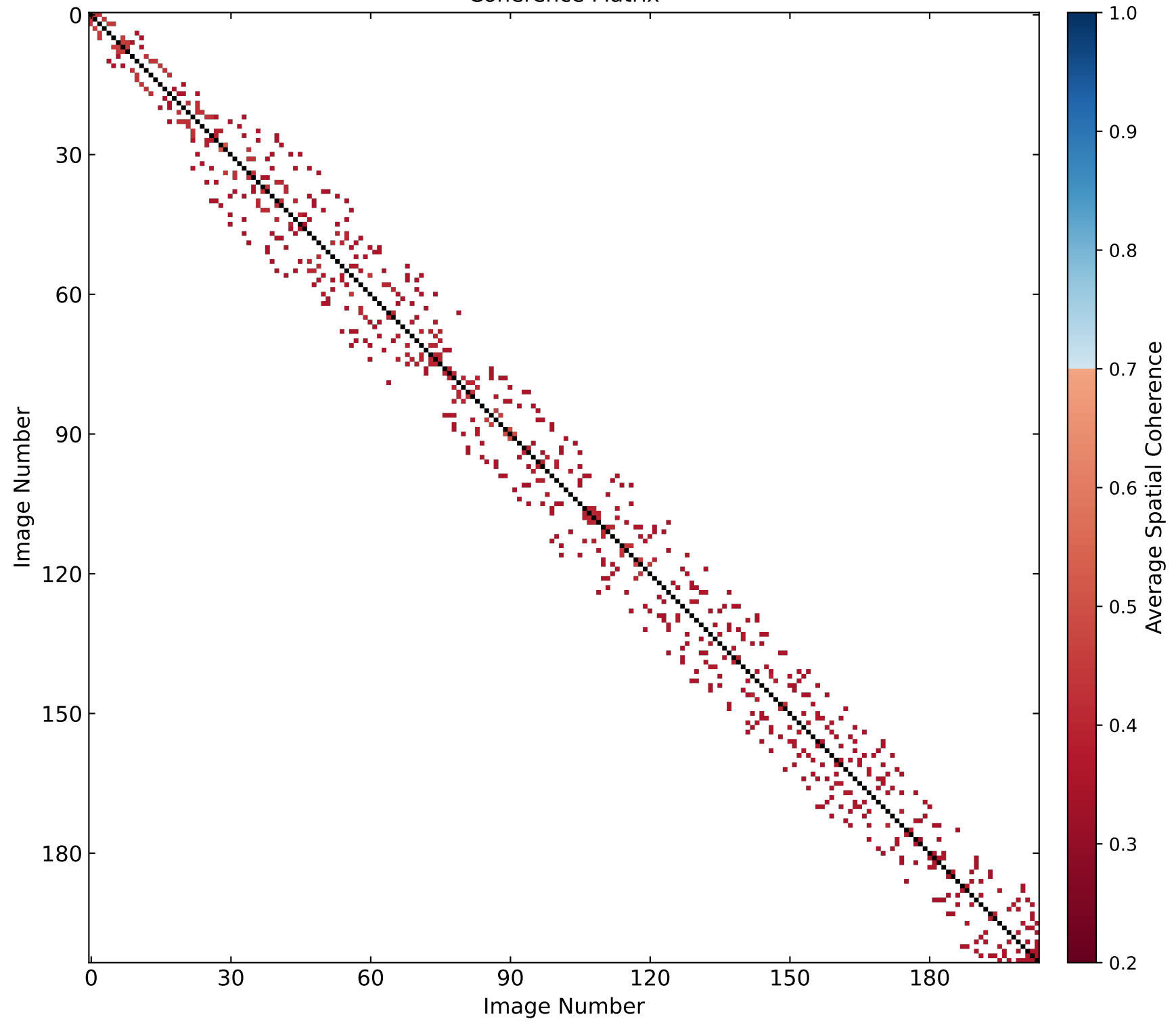
Coherence Matrix
