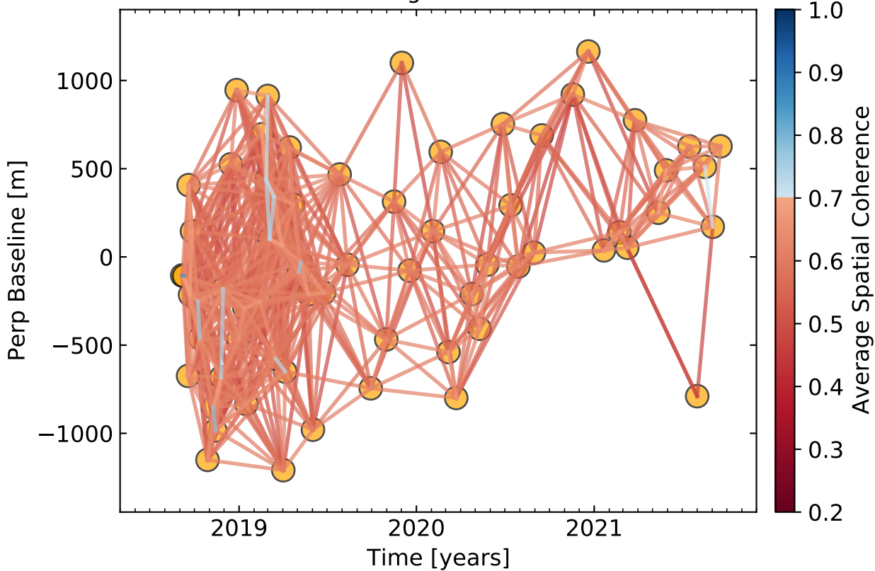
Interferogram Network
