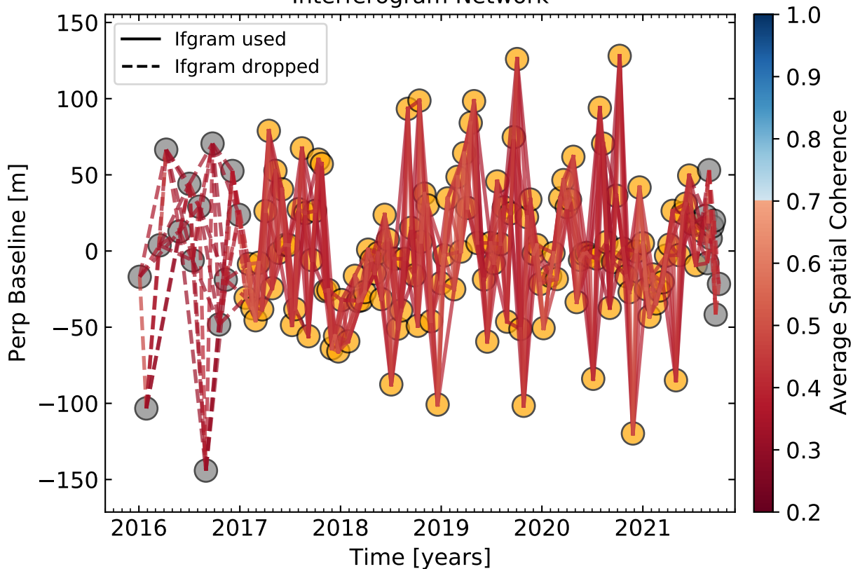
Interferogram Network
