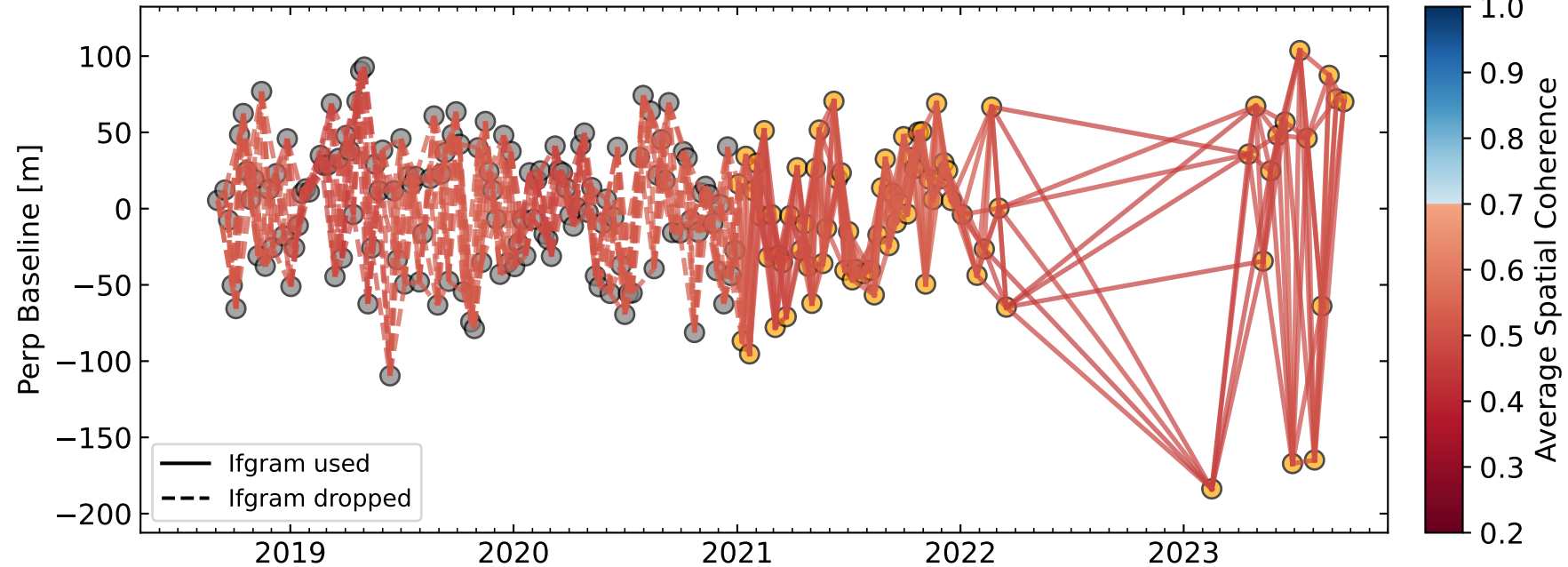
Interferogram Network
