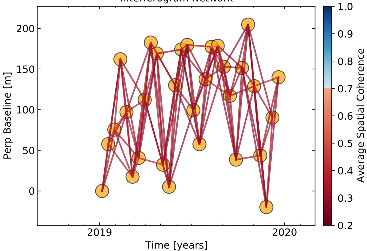
Interferogram Network
