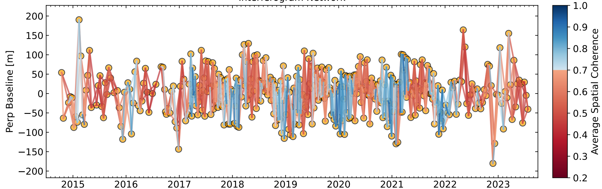
Interferogram Network
