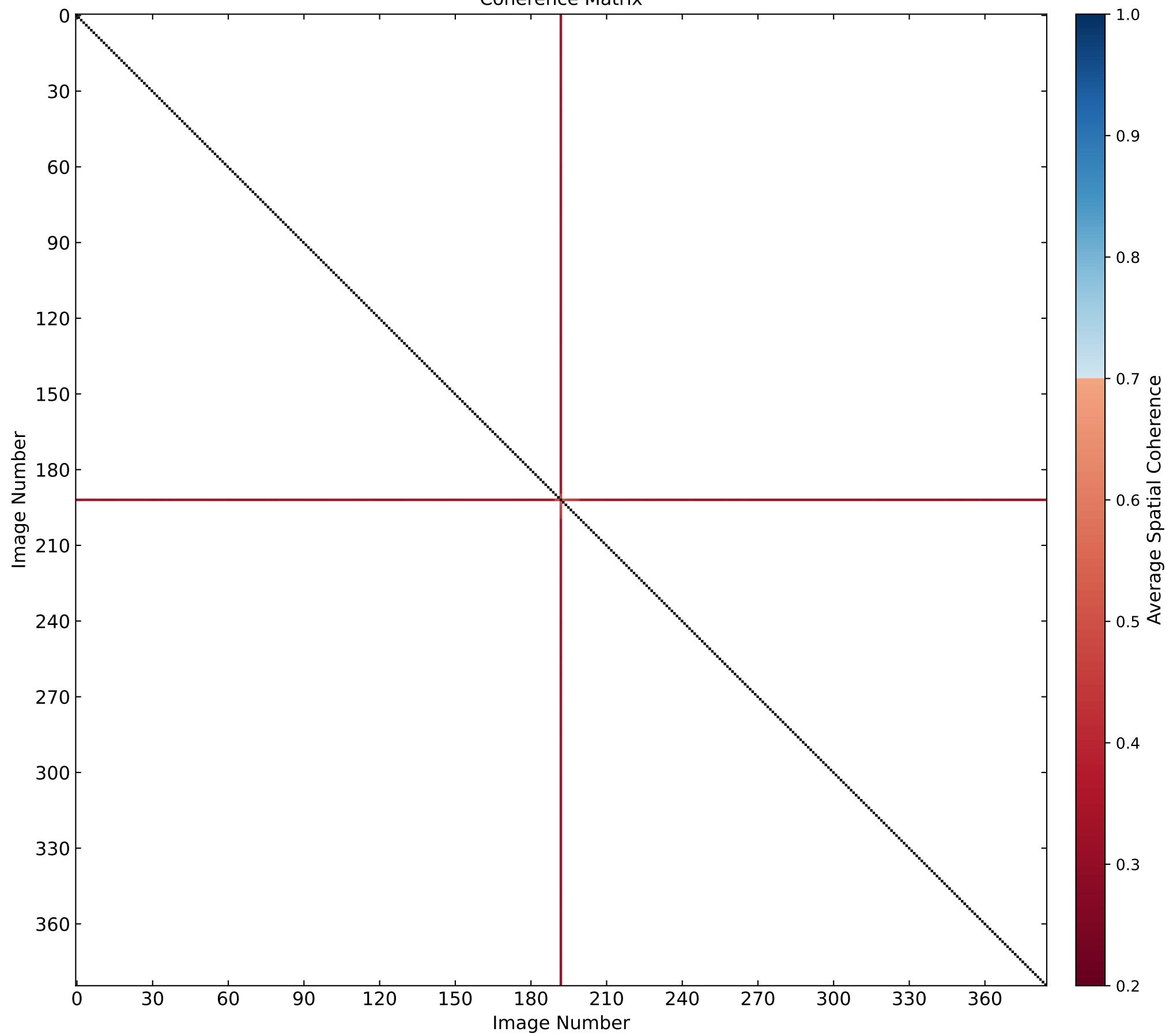
Coherence Matrix
