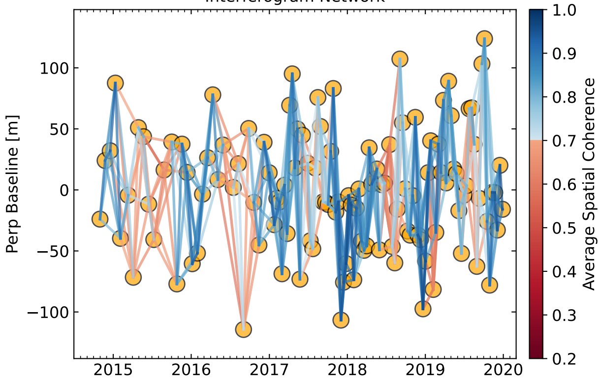
Interferogram Network
