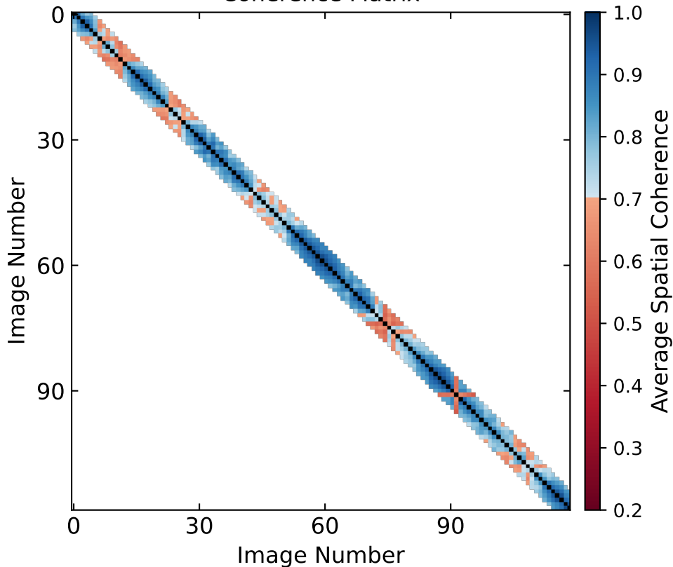
Coherence Matrix
