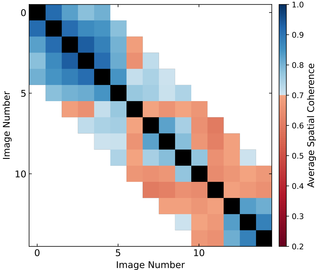
Coherence Matrix
