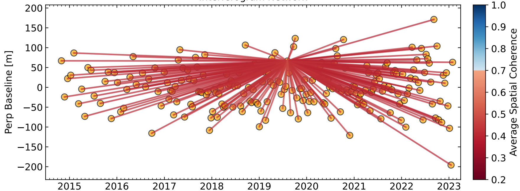
Interferogram Network
