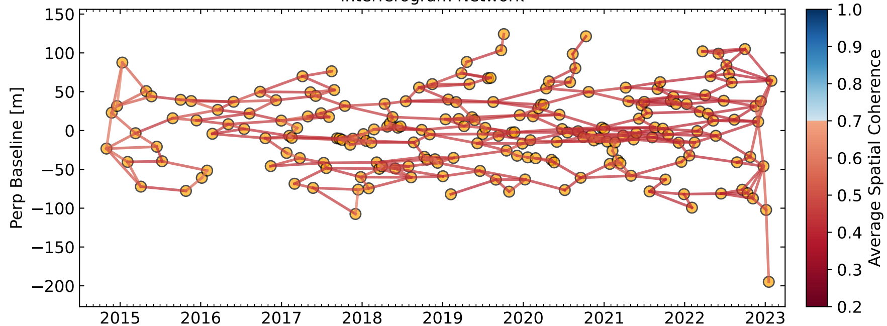
Interferogram Network
