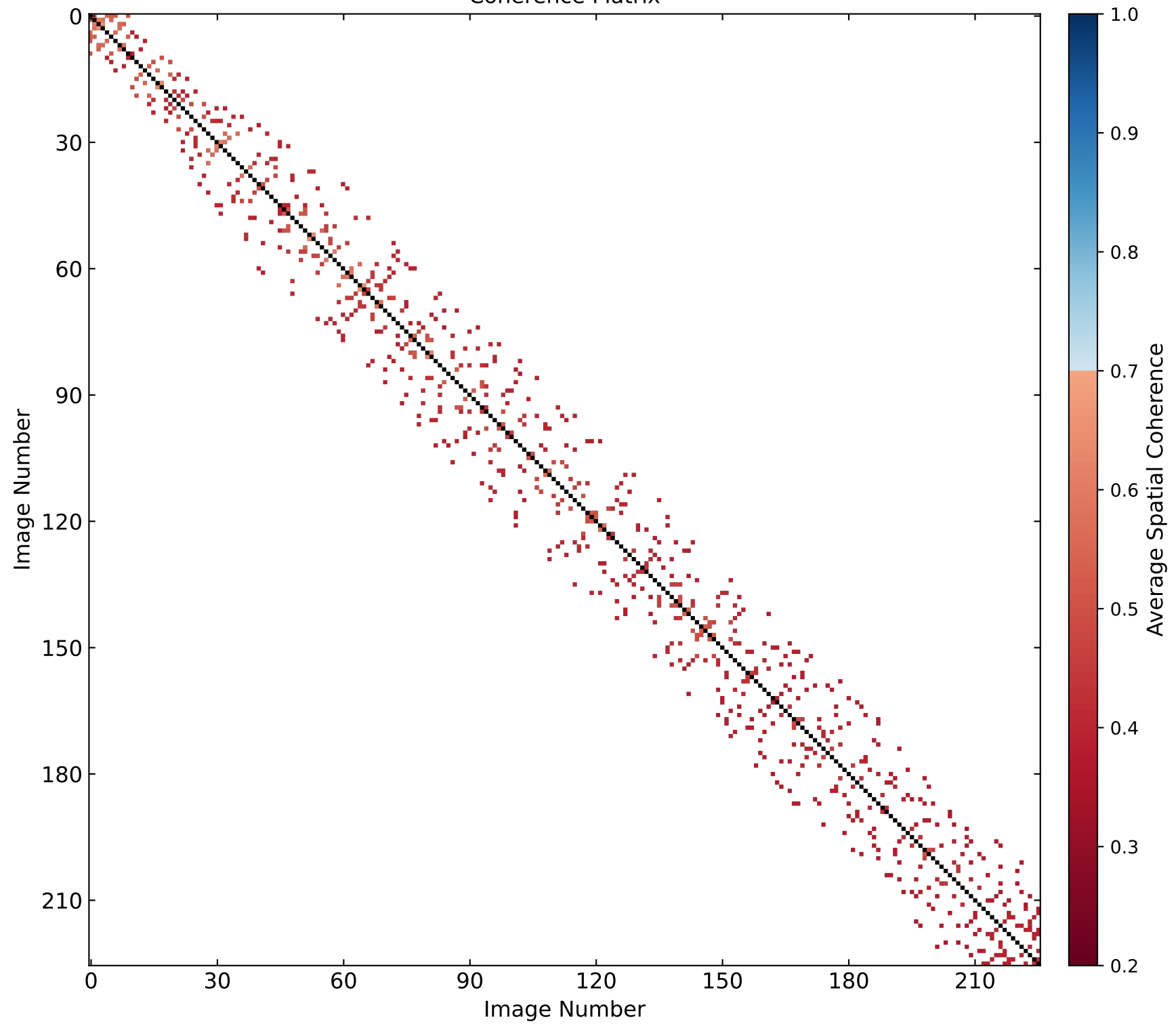
Coherence Matrix
